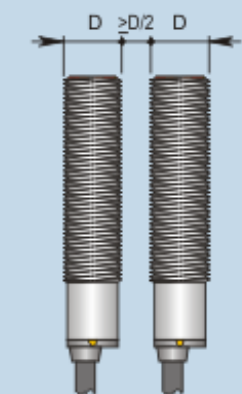
Side by side mounting
